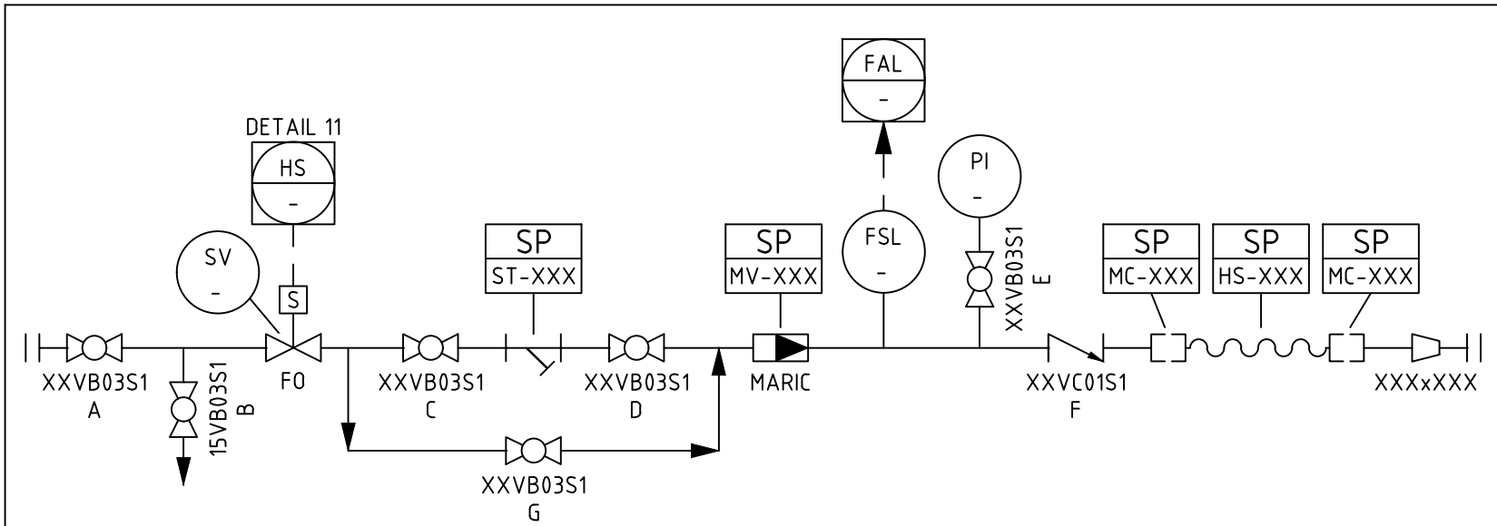
GLAND WATER DETAIL 1 SOLENOID VALVE AND FLOW SWITCH (REFER TABLE FOR SIZING AND INFORMATION)
