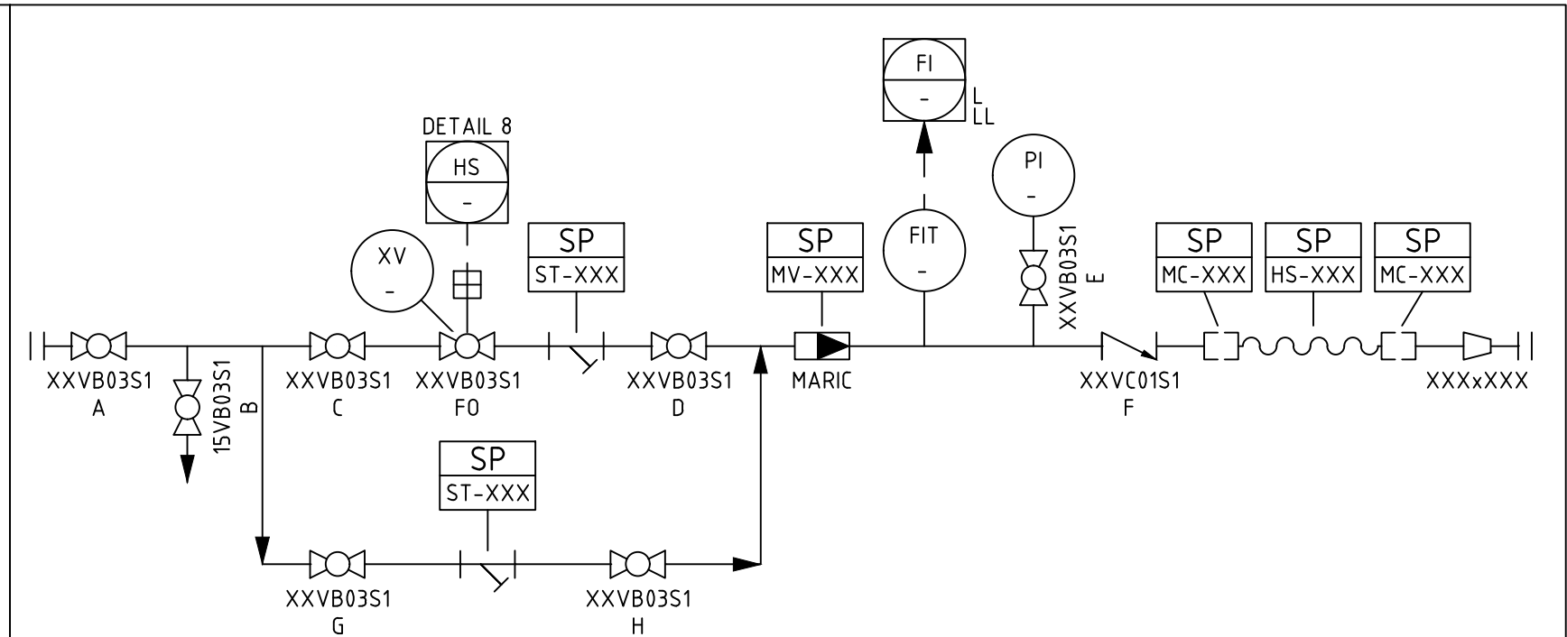
GLAND WATER DETAIL 3 BALL VALVE AND FLOW TRANSMITTER (DN32 & ABOVE) (REFER TABLE FOR SIZING AND INFORMATION)
