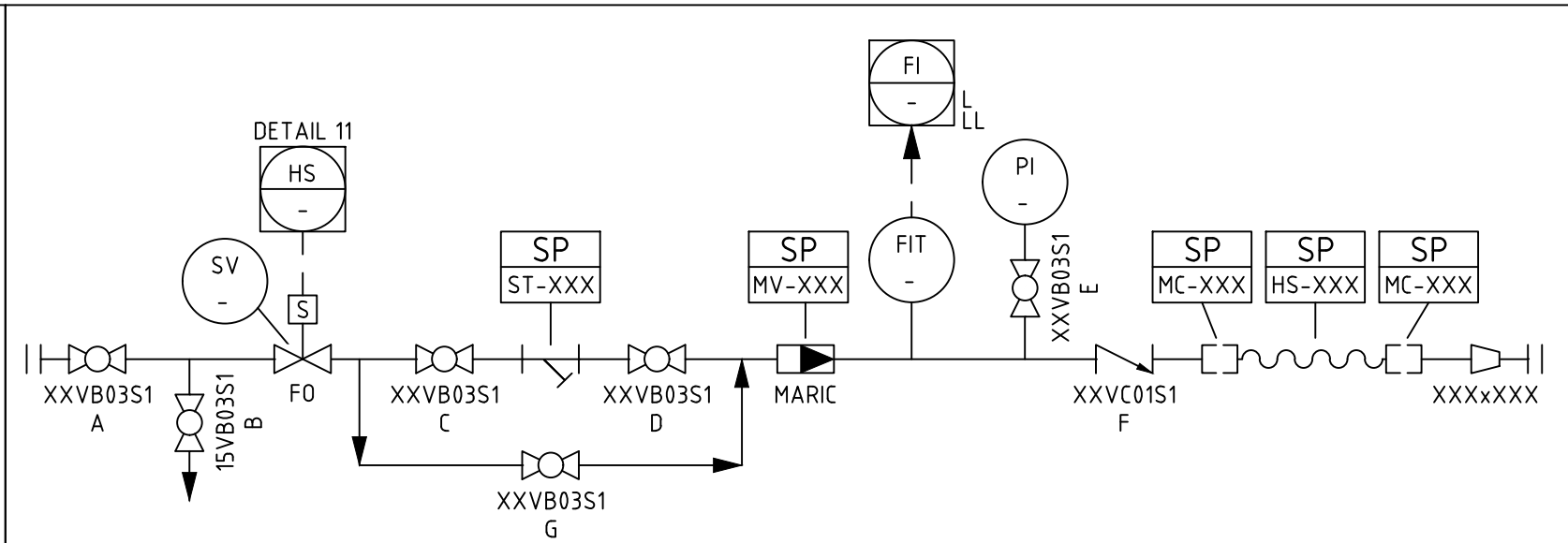
GLAND WATER DETAIL 2 SOLENOID VALVE AND FLOW TRANSMITTER (DN25 & UNDER) (REFER TABLE FOR SIZING AND INFORMATION)
